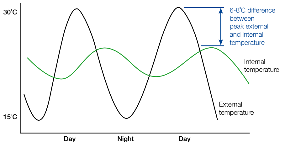
Typical masonry thermal mass/phasing effect (actual performance depends upon material and thickness)
